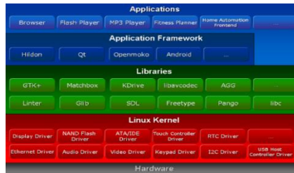
Linux Software Stack
