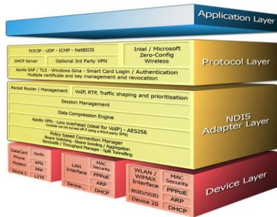
Windows Software Stack
