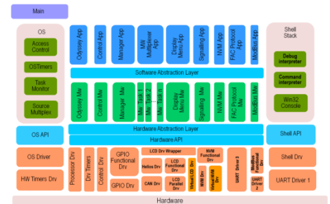
Odyssey Software Stack
